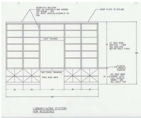
Office Wall Unit Shop Drawing
